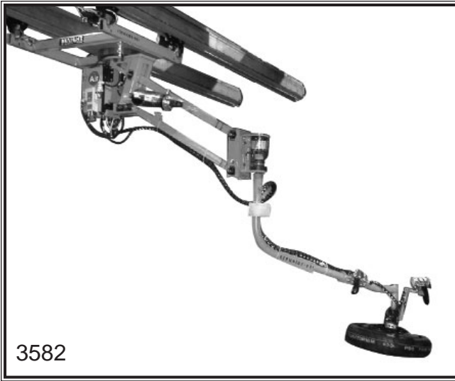
Expanding mandrel fixture to load spare tire.
