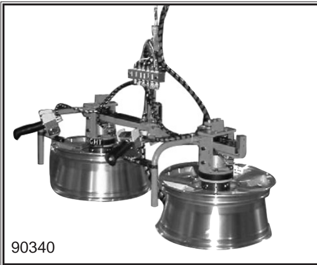
Dual expanding mandrel fixture to transfer rims.
